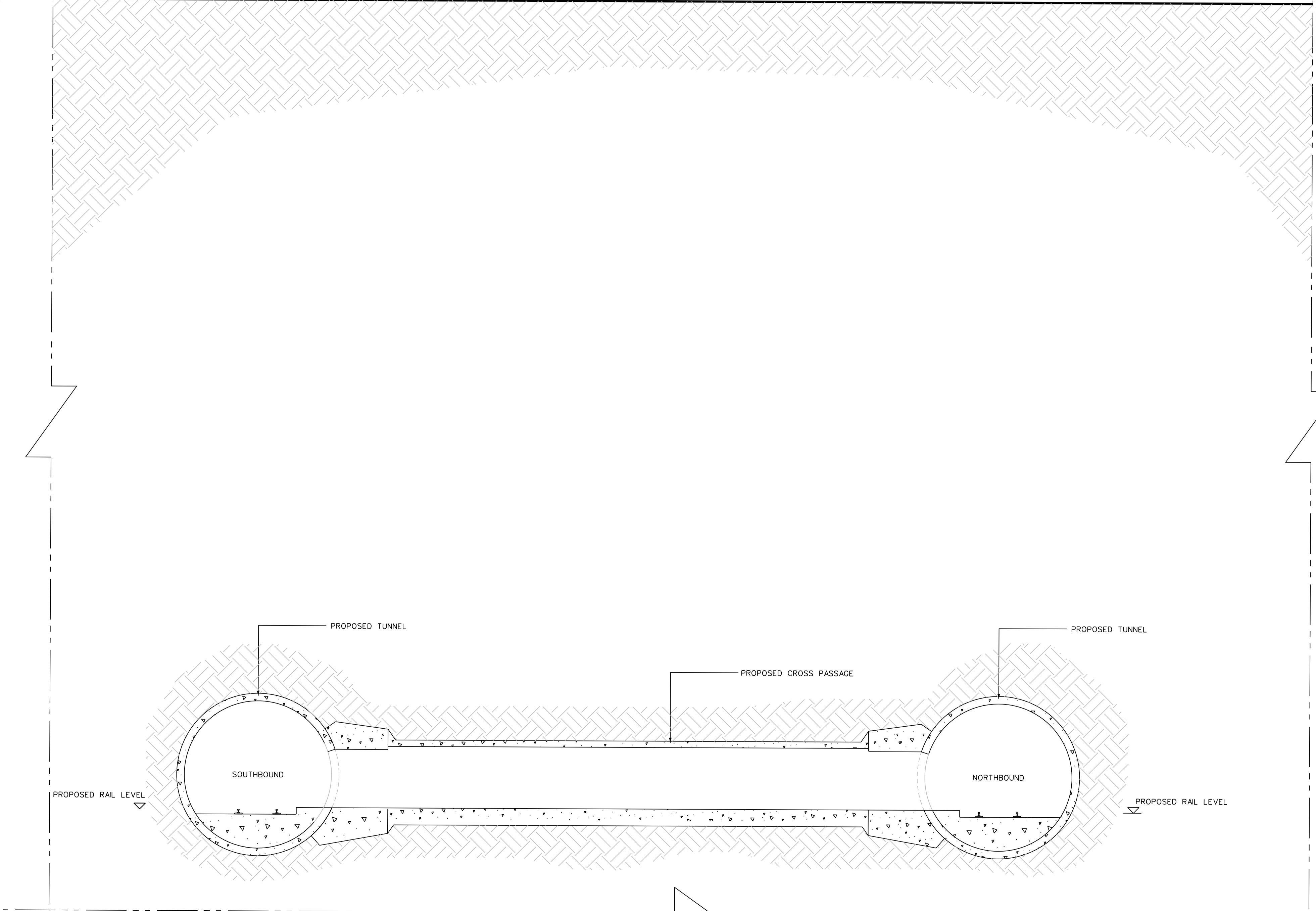
CROSS SECTION 06-05 SCALE 1:100
