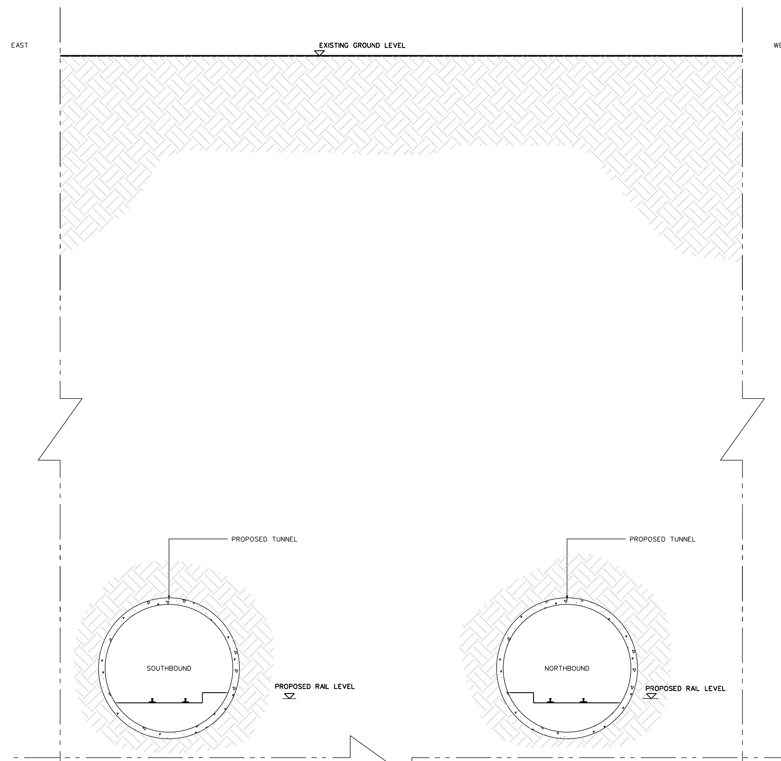
CROSS SECTION 07-04 SCALE 1:100
