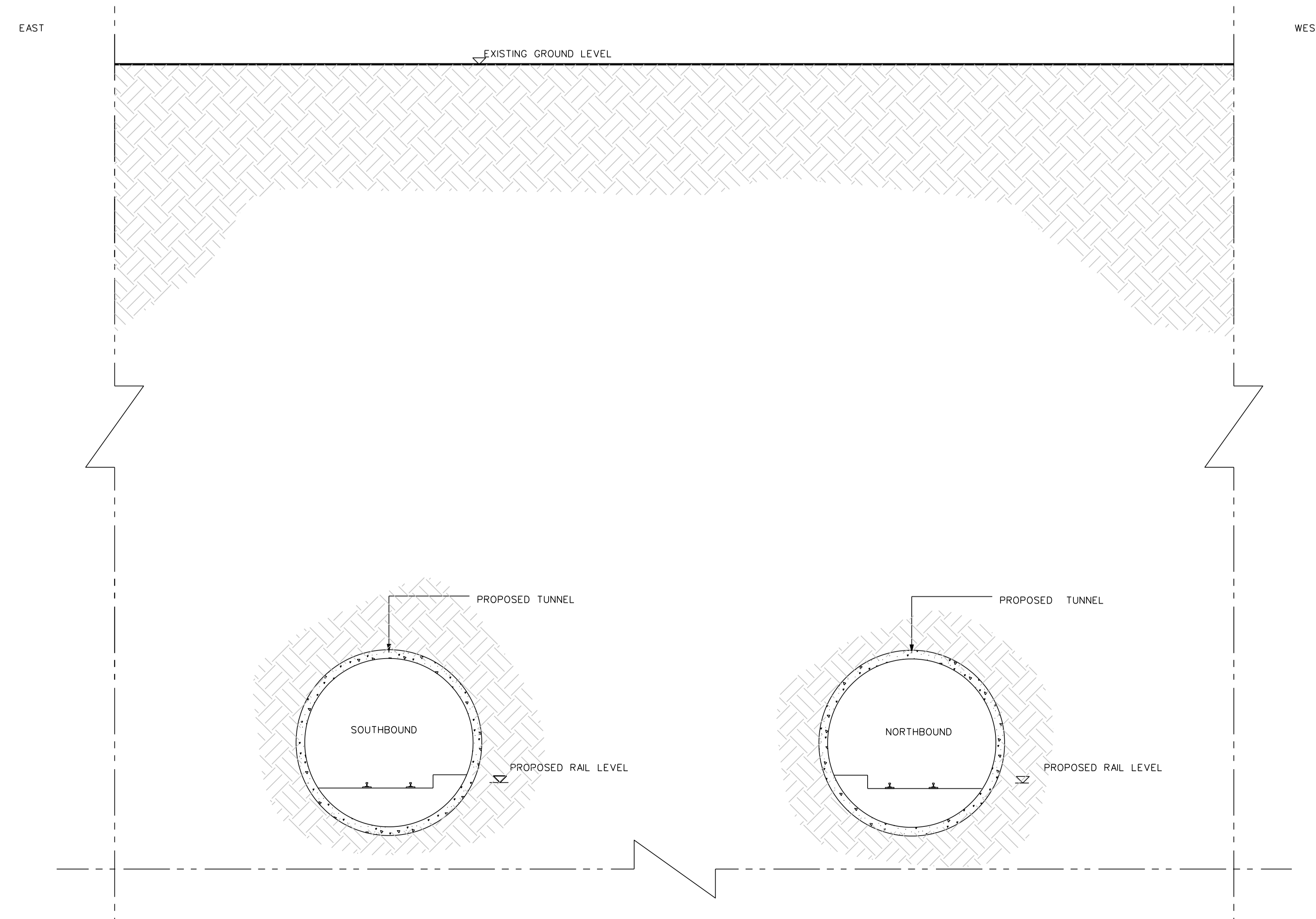
CROSS SECTION 03-01 SCALE 1:100
