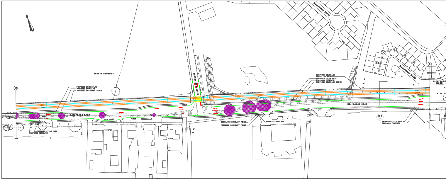
PLAN Scale 1:100
