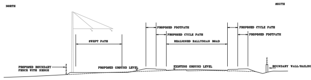
PROPOSED CROSS SECTION 14-A 1:100
